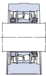
Locating bearing unit SYT .. FTS
